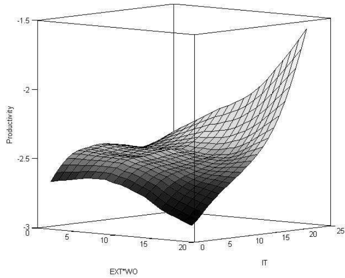
Figure 4: Level Plots of Fitted Values from Regression of Productivity on External Focus, Workplace Organization, and Information Technology
