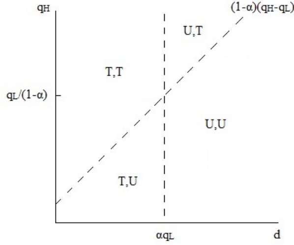
Figure 4: Lemma 1
