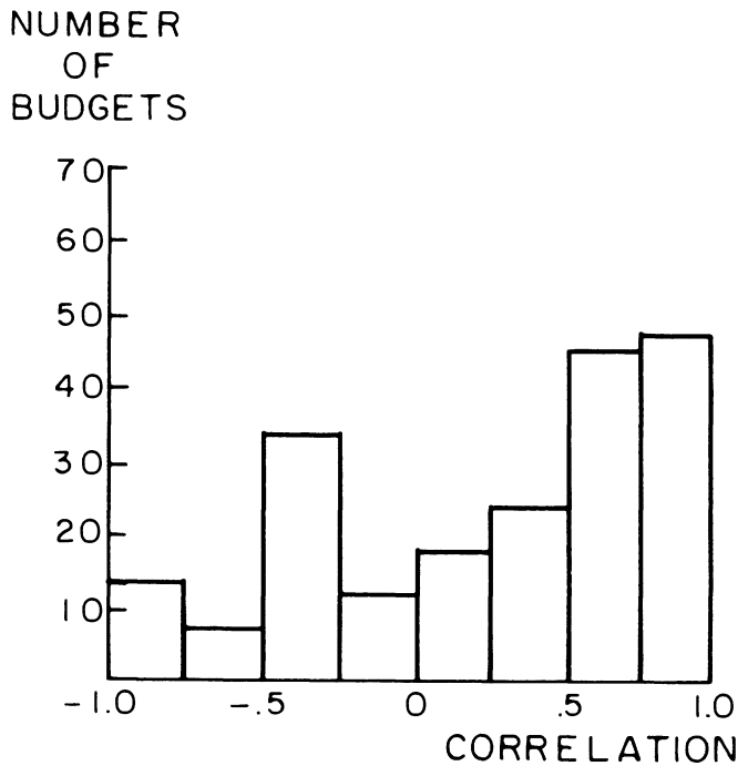
3 Prediction based on lottery order
