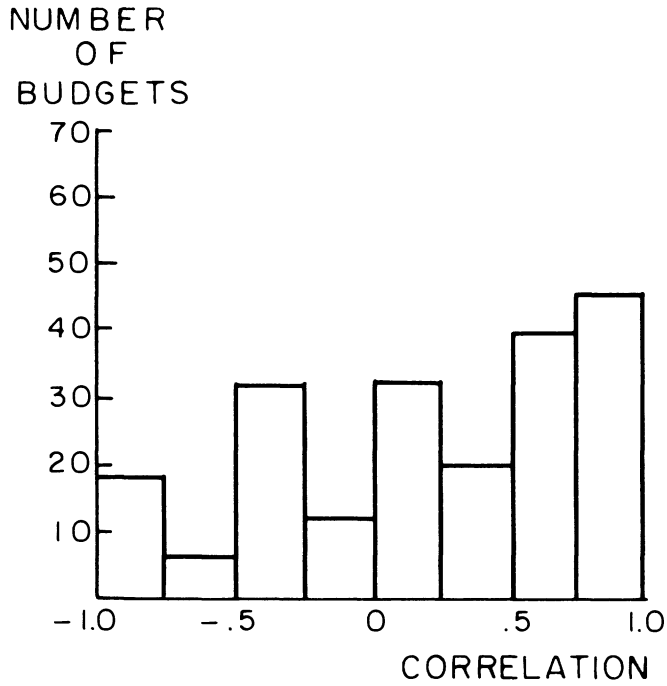
1 Prediction based on reservation price
