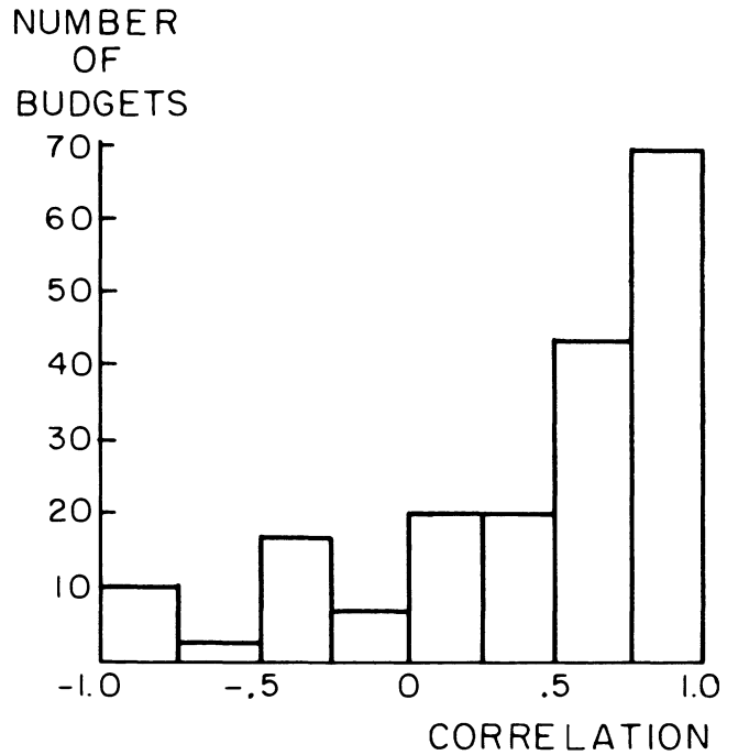
2 Prediction based on purchase probabilities
